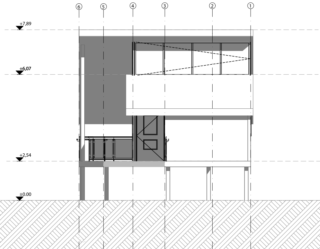
1. FACHADA PRINCIPAL 1:100
